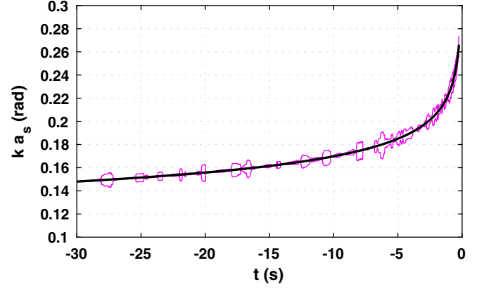
FIG. 3. Observed gravitational wave GW170817 gravitational quadrupole size parameter ka_s as a function of time. Solid curve is for fit to data, with thin gray (magenta in color prints) curves indicating error in ka_s that would correspond to the two-standard-deviation error in f_{gw} of Fig. 2(b). Coalescence is at t = 0 .
